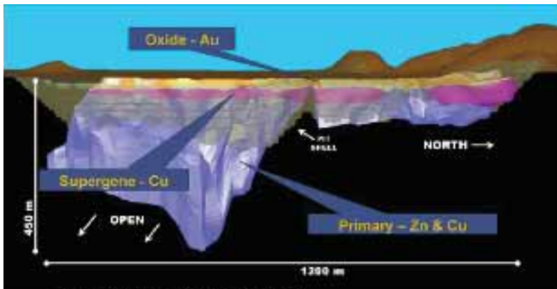
Bisha VMS Cross Section
